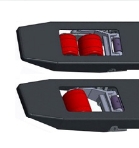
Single / Tandem Load Wheels
